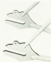
TRACK ENDS long-slot with dogs for chain adjusters and mudguard eyes
