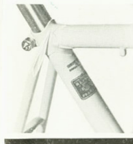
HEAD ASSEMBLY SHOWING LUG AND CROWN DESIGN
